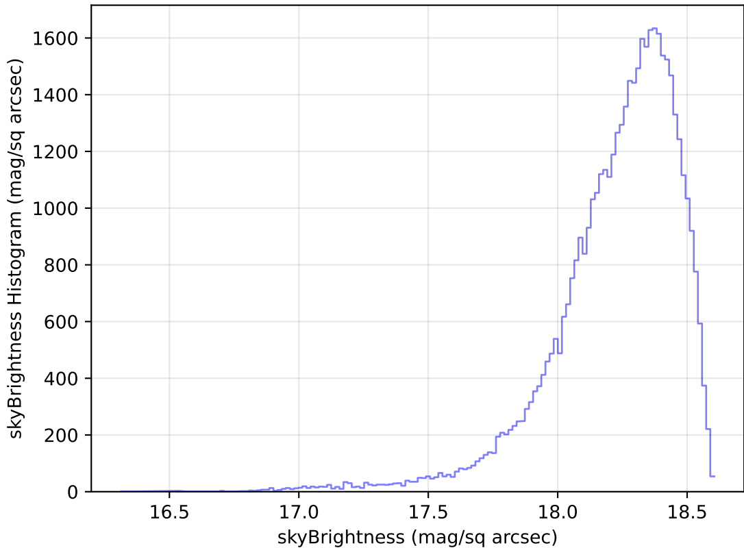
too_elab_r64_d3_gz_v3.4_10yrs Yr 1 y band: skyBrightness Histogram
