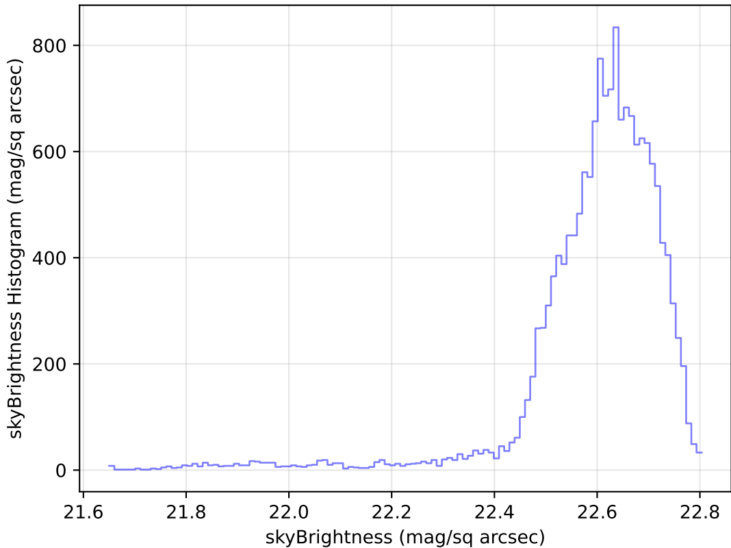
too_elab_r64_d3_gz_v3.4_10yrs Yr 1 u band: skyBrightness Histogram
