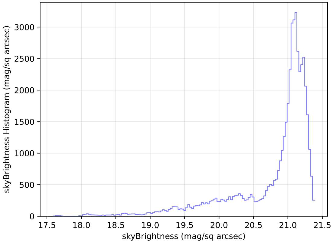
too_elab_r64_d3_gz_v3.4_10yrs Yr 1 r band: skyBrightness Histogram
