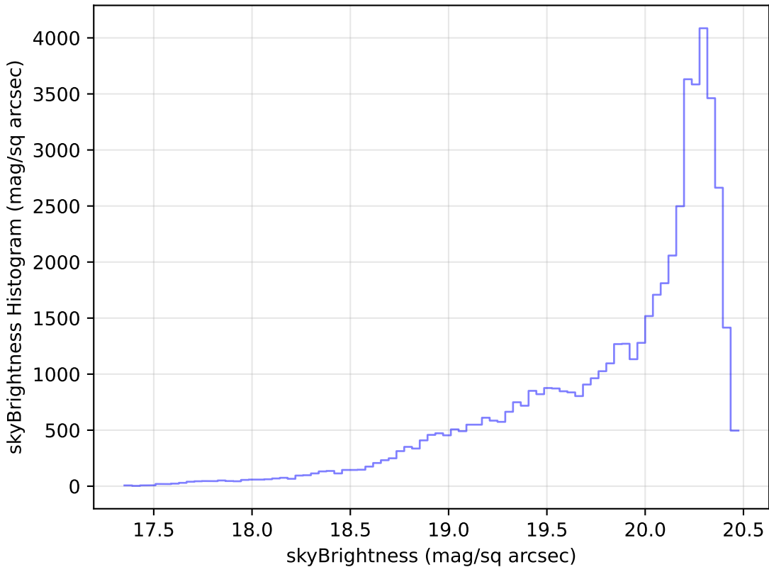
too_elab_r64_d3_gz_v3.4_10yrs Yr 1 i band: skyBrightness Histogram
