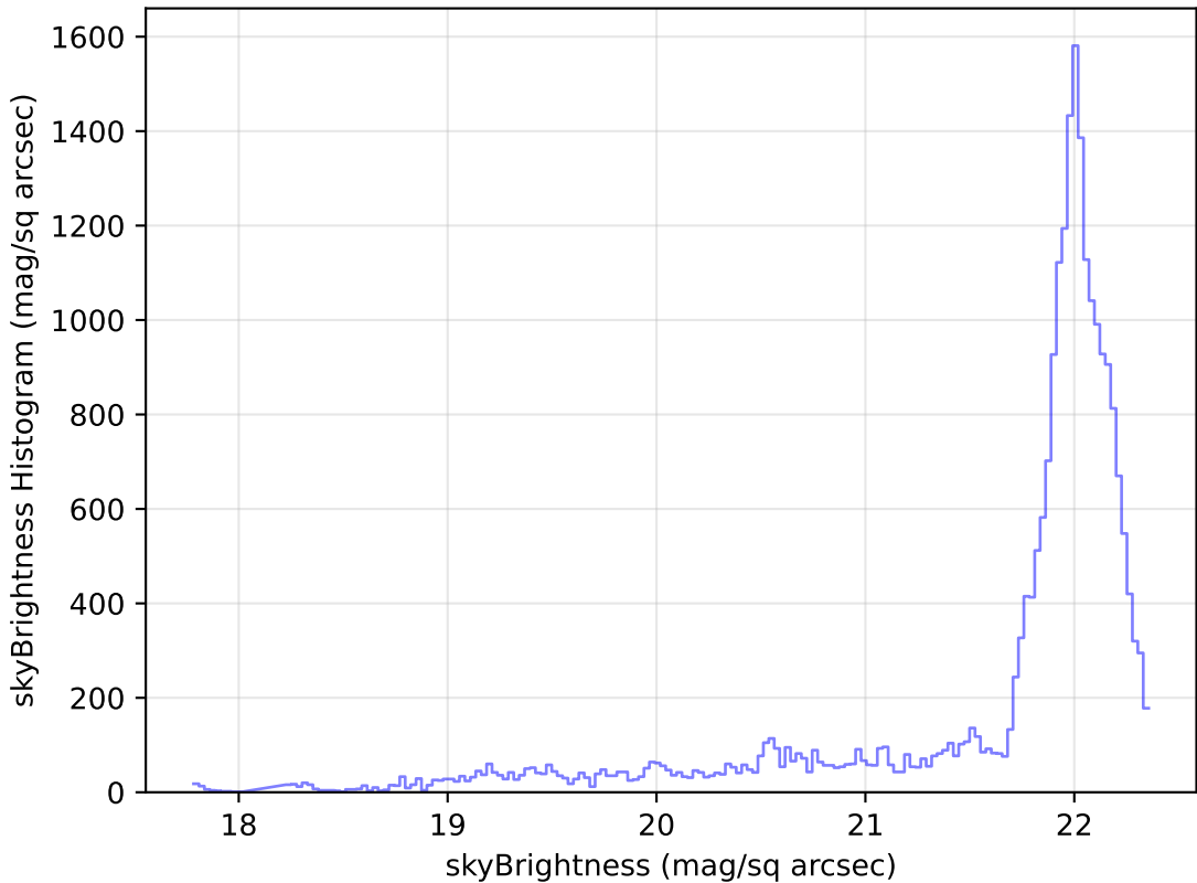
too_elab_r64_d3_gz_v3.4_10yrs Yr 1 g band: skyBrightness Histogram
