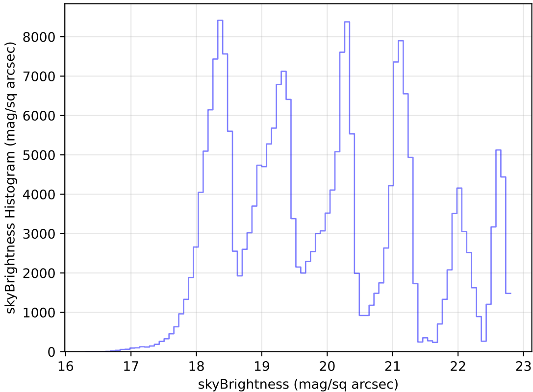
too_elab_r64_d3_gz_v3.4_10yrs Yr 1 all bands: skyBrightness Histogram
