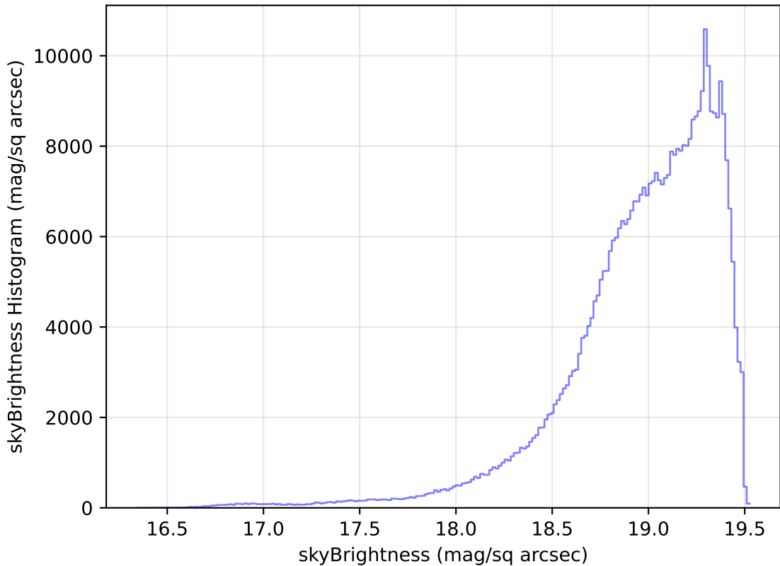
too_elab_r64_d3_gz_v3.4_10yrs WFD z band: skyBrightness Histogram
