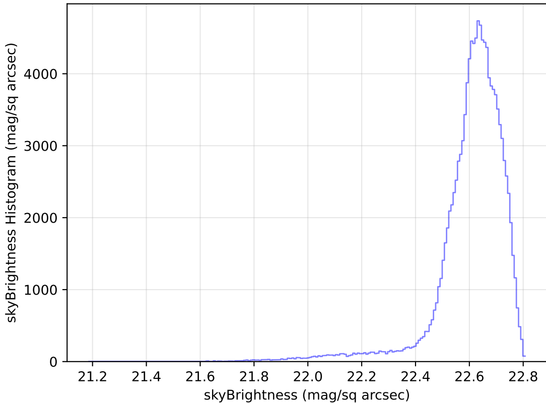
too_elab_r64_d3_gz_v3.4_10yrs WFD u band: skyBrightness Histogram
