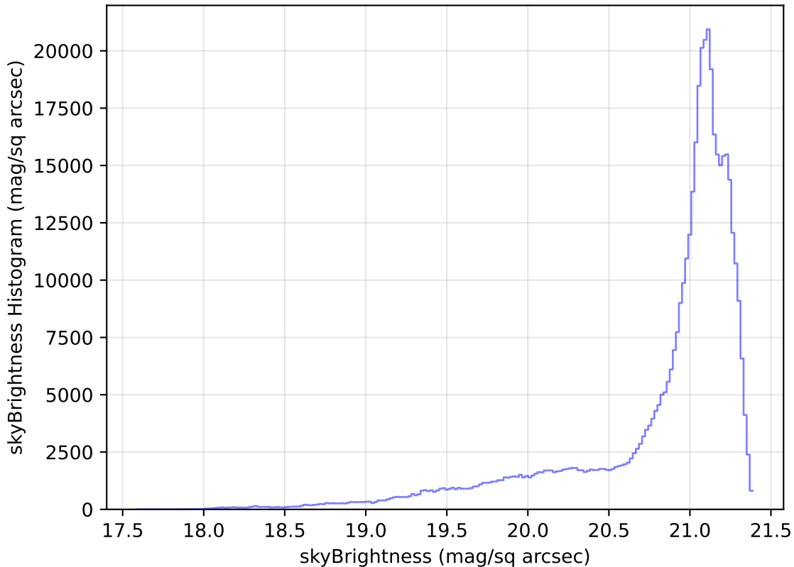
too_elab_r64_d3_gz_v3.4_10yrs WFD r band: skyBrightness Histogram
