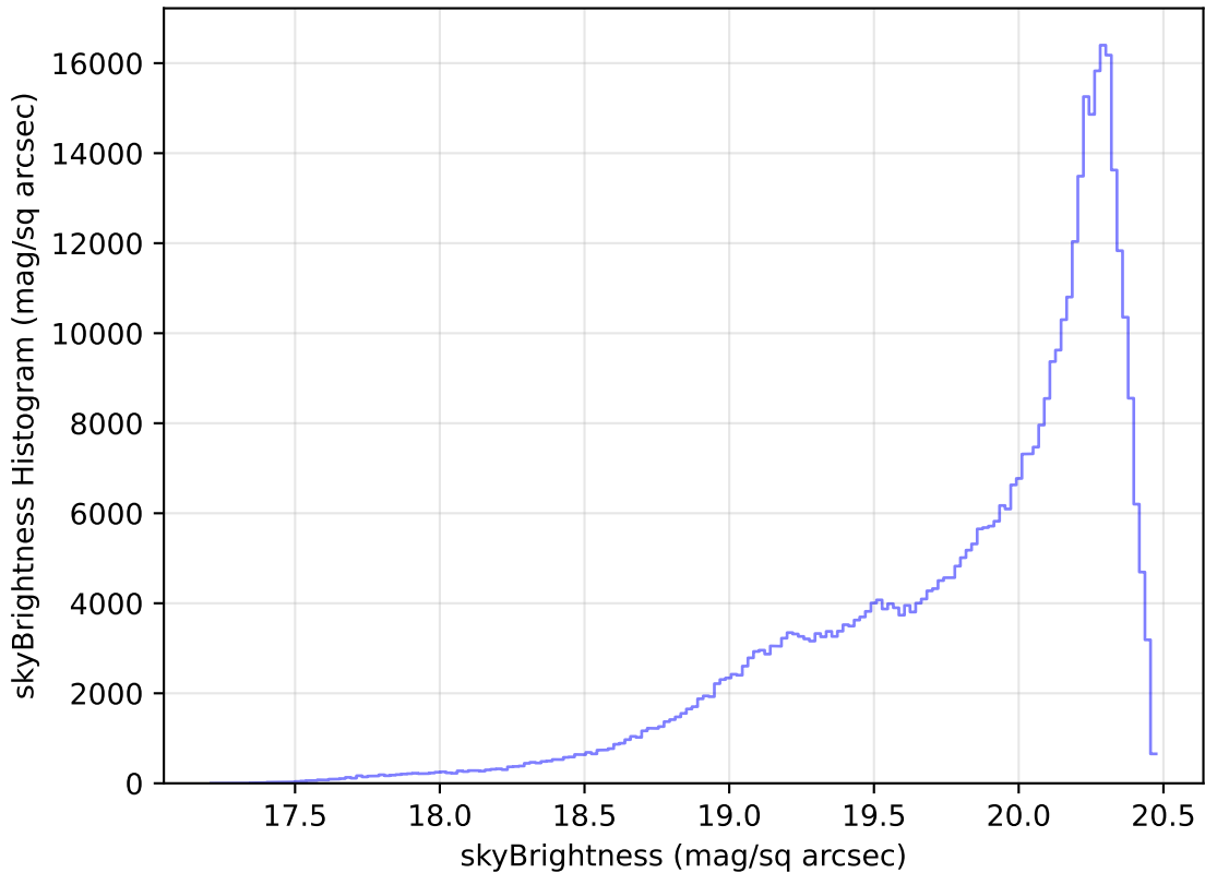
too_elab_r64_d3_gz_v3.4_10yrs WFD i band: skyBrightness Histogram
