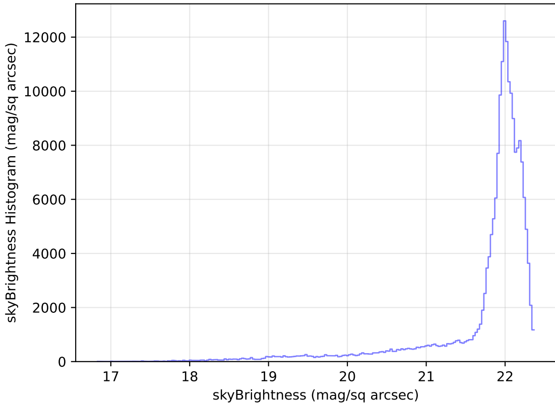
too_elab_r64_d3_gz_v3.4_10yrs WFD g band: skyBrightness Histogram
