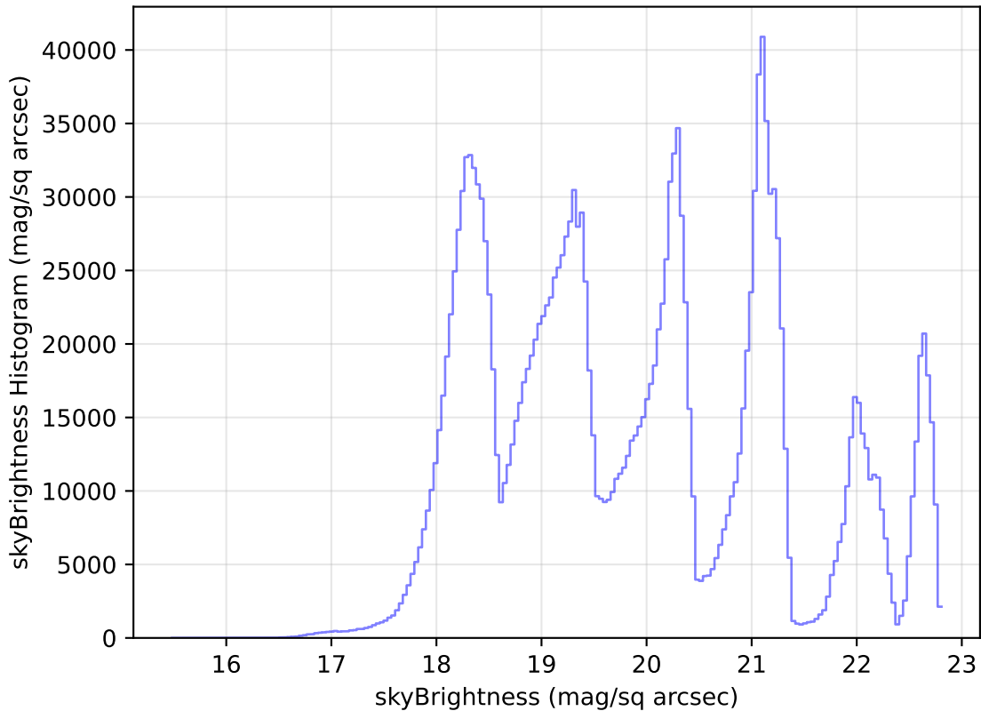
too_elab_r64_d3_gz_v3.4_10yrs WFD all bands: skyBrightness Histogram
