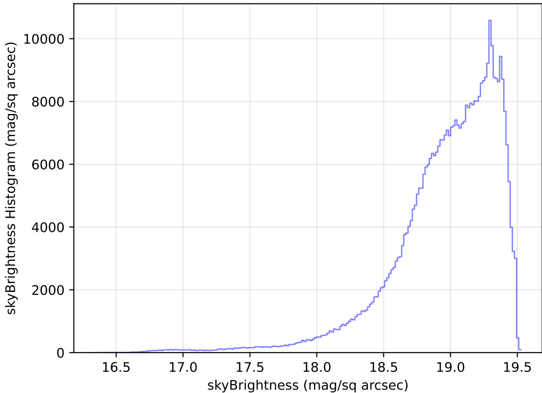
too_elab_r64_d3_gz_v3.4_10yrs All sky z band: skyBrightness Histogram
