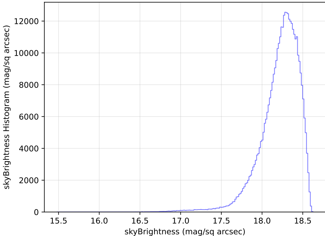
too_elab_r64_d3_gz_v3.4_10yrs All sky y band: skyBrightness Histogram
