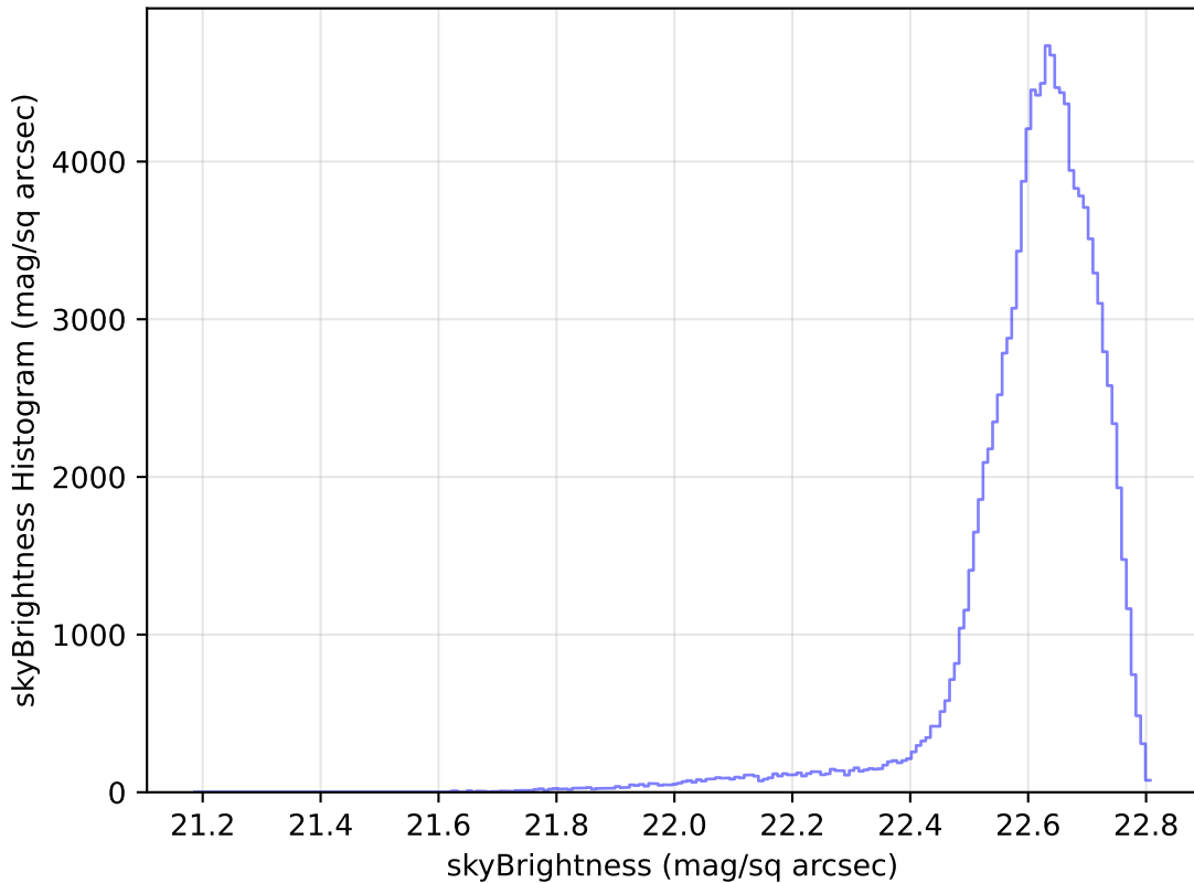
too_elab_r64_d3_gz_v3.4_10yrs All sky u band: skyBrightness Histogram
