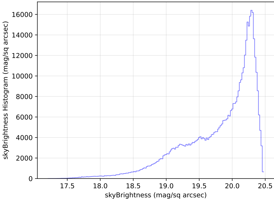
too_elab_r64_d3_gz_v3.4_10yrs All sky i band: skyBrightness Histogram
