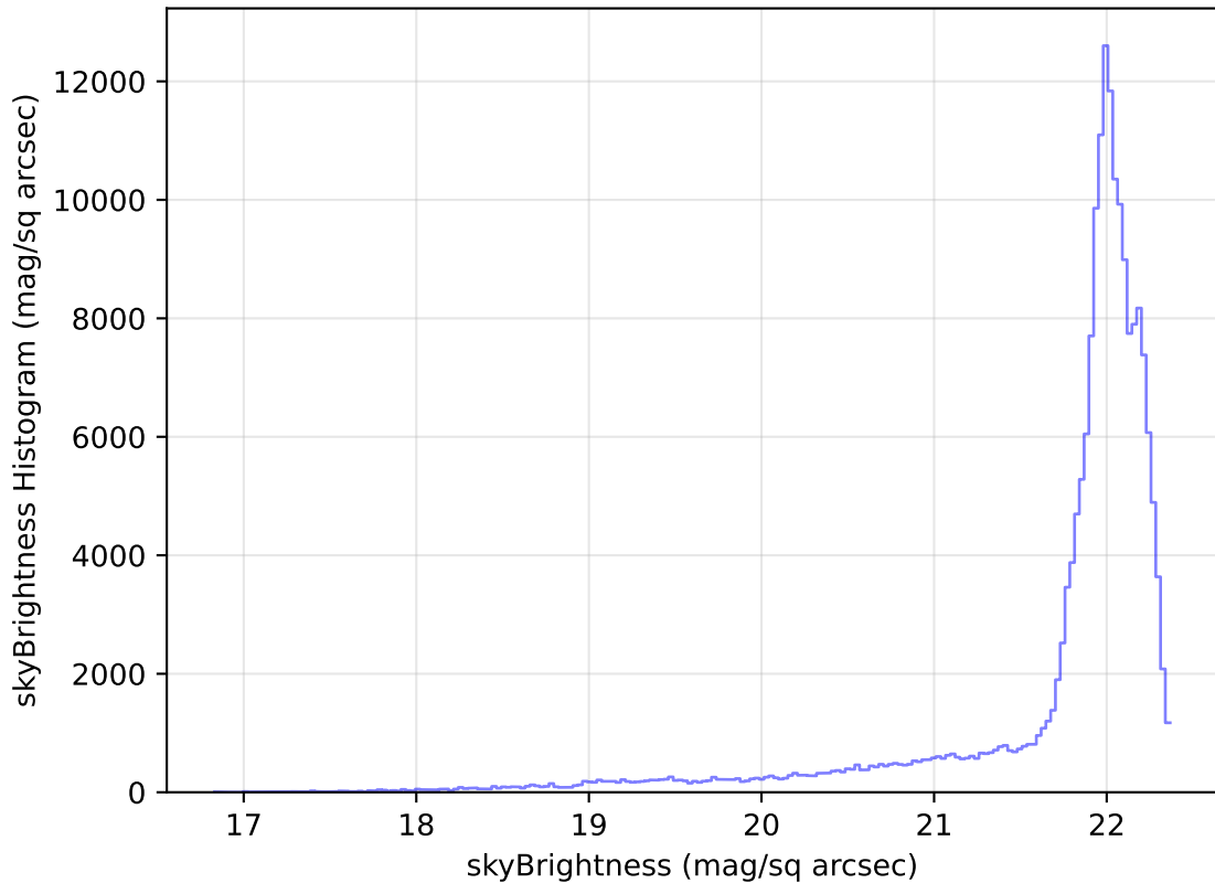
too_elab_r64_d3_gz_v3.4_10yrs All sky g band: skyBrightness Histogram
