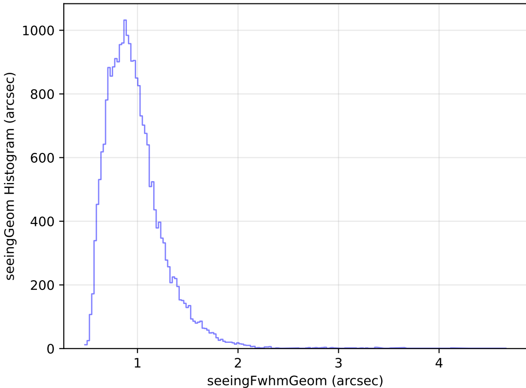
too_elab_r64_d3_gz_v3.4_10yrs Yr 1 g band: seeingGeom Histogram
