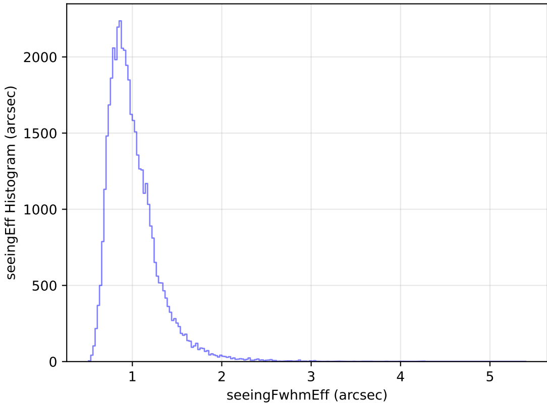
too_elab_r64_d3_gz_v3.4_10yrs Yr 1 z band: seeingEff Histogram
