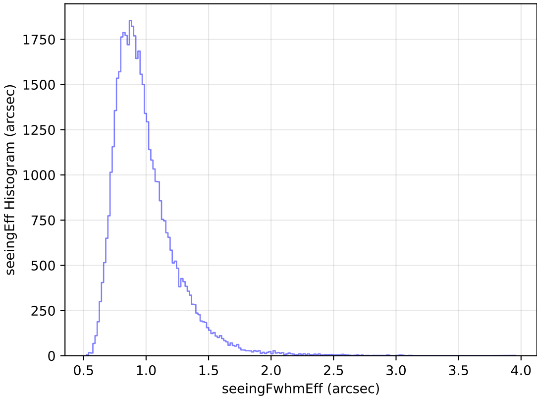
too_elab_r64_d3_gz_v3.4_10yrs Yr 1 y band: seeingEff Histogram
