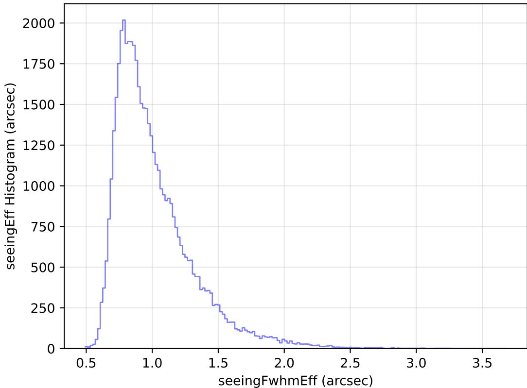
too_elab_r64_d3_gz_v3.4_10yrs Yr 1 r band: seeingEff Histogram
