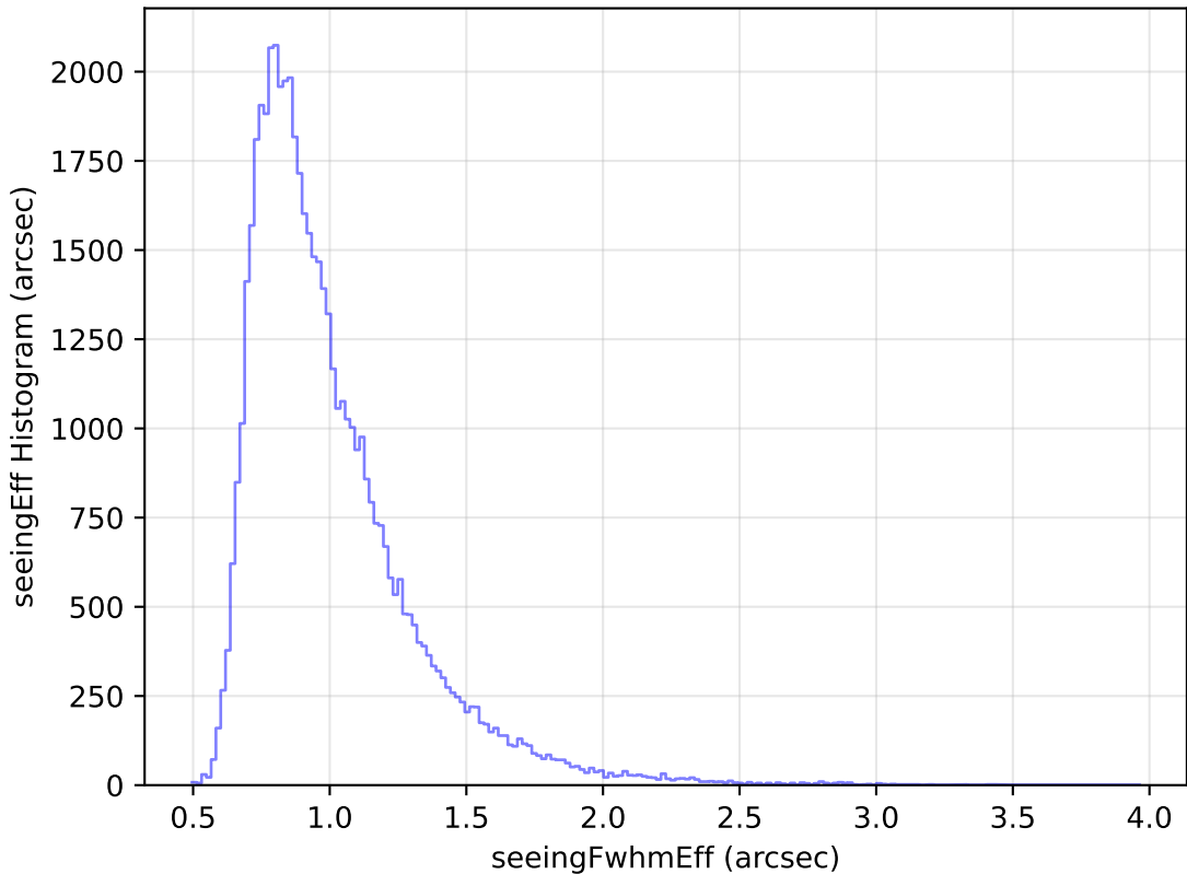
too_elab_r64_d3_gz_v3.4_10yrs Yr 1 i band: seeingEff Histogram
