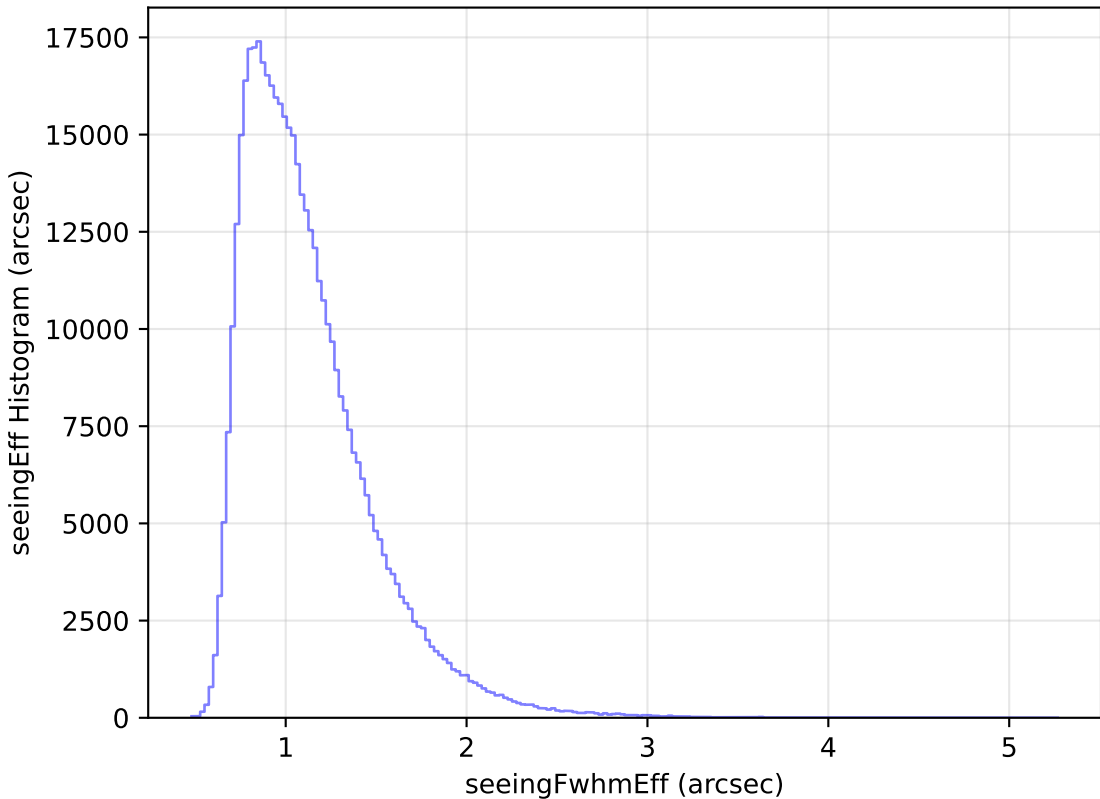
too_elab_r64_d3_gz_v3.4_10yrs WFD r band: seeingEff Histogram
