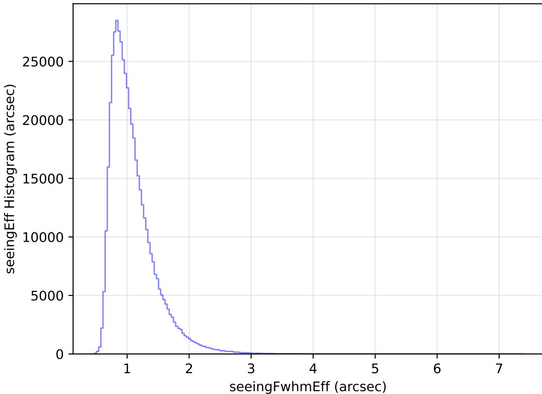
too_elab_r64_d3_gz_v3.4_10yrs WFD i band: seeingEff Histogram
