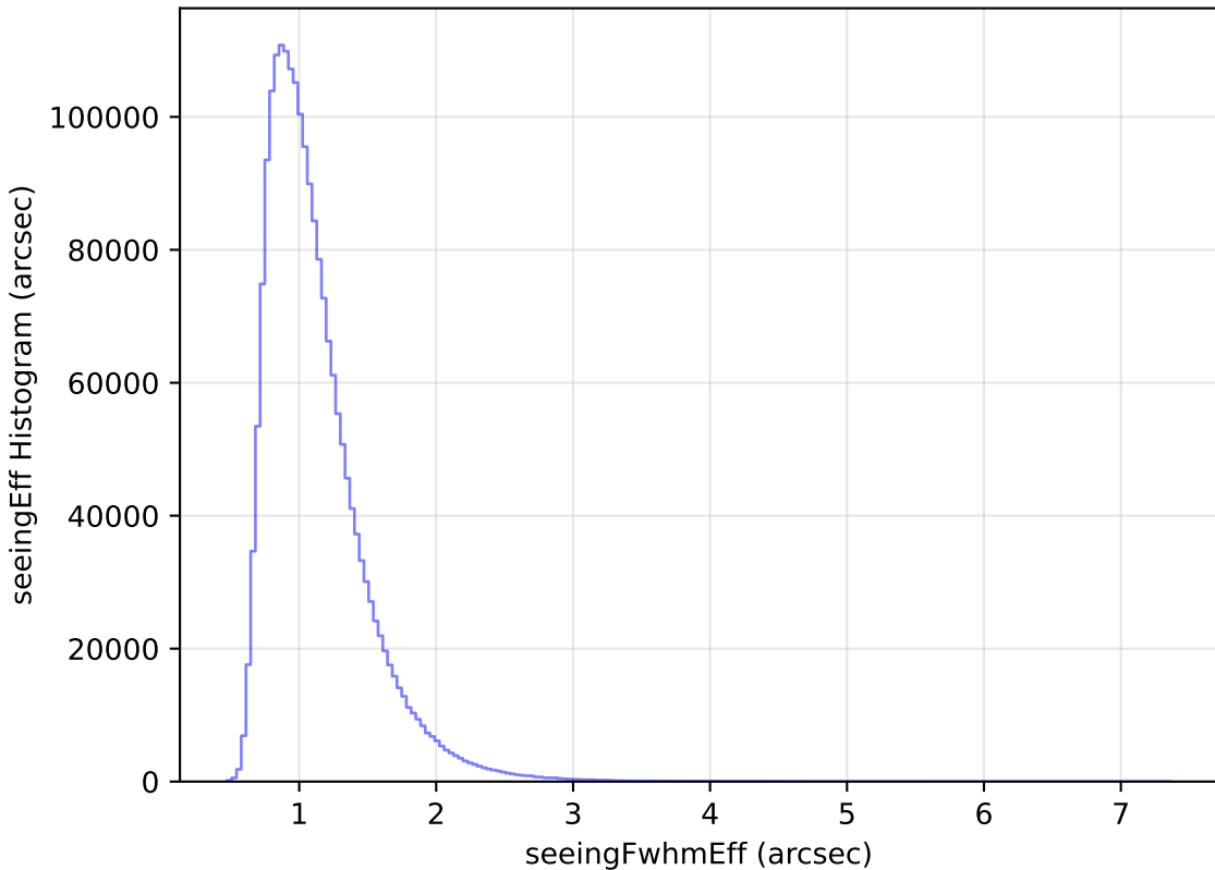
too_elab_r64_d3_gz_v3.4_10yrs WFD all bands: seeingEff Histogram
