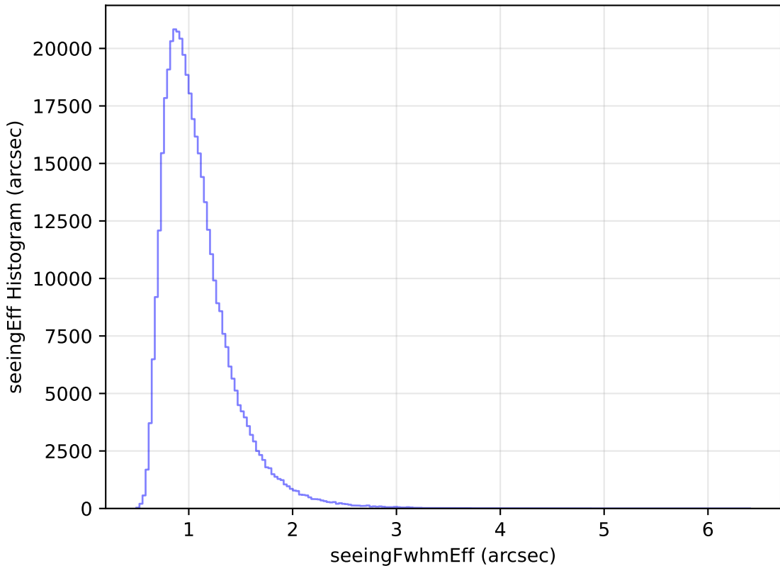
too_elab_r64_d3_gz_v3.4_10yrs All sky z band: seeingEff Histogram
