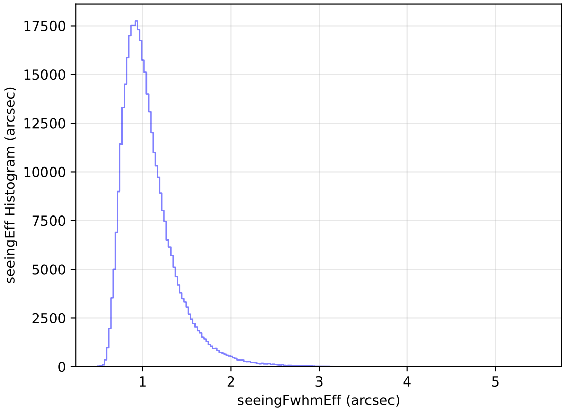
too_elab_r64_d3_gz_v3.4_10yrs All sky y band: seeingEff Histogram
