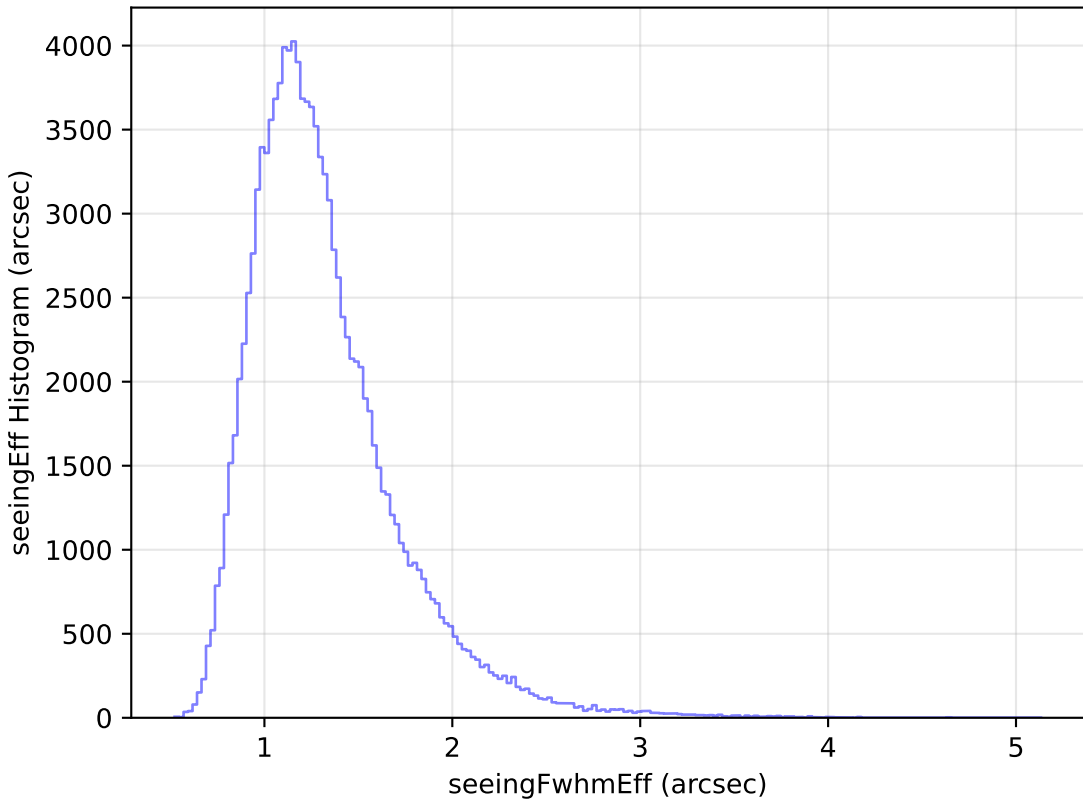
too_elab_r64_d3_gz_v3.4_10yrs All sky u band: seeingEff Histogram
