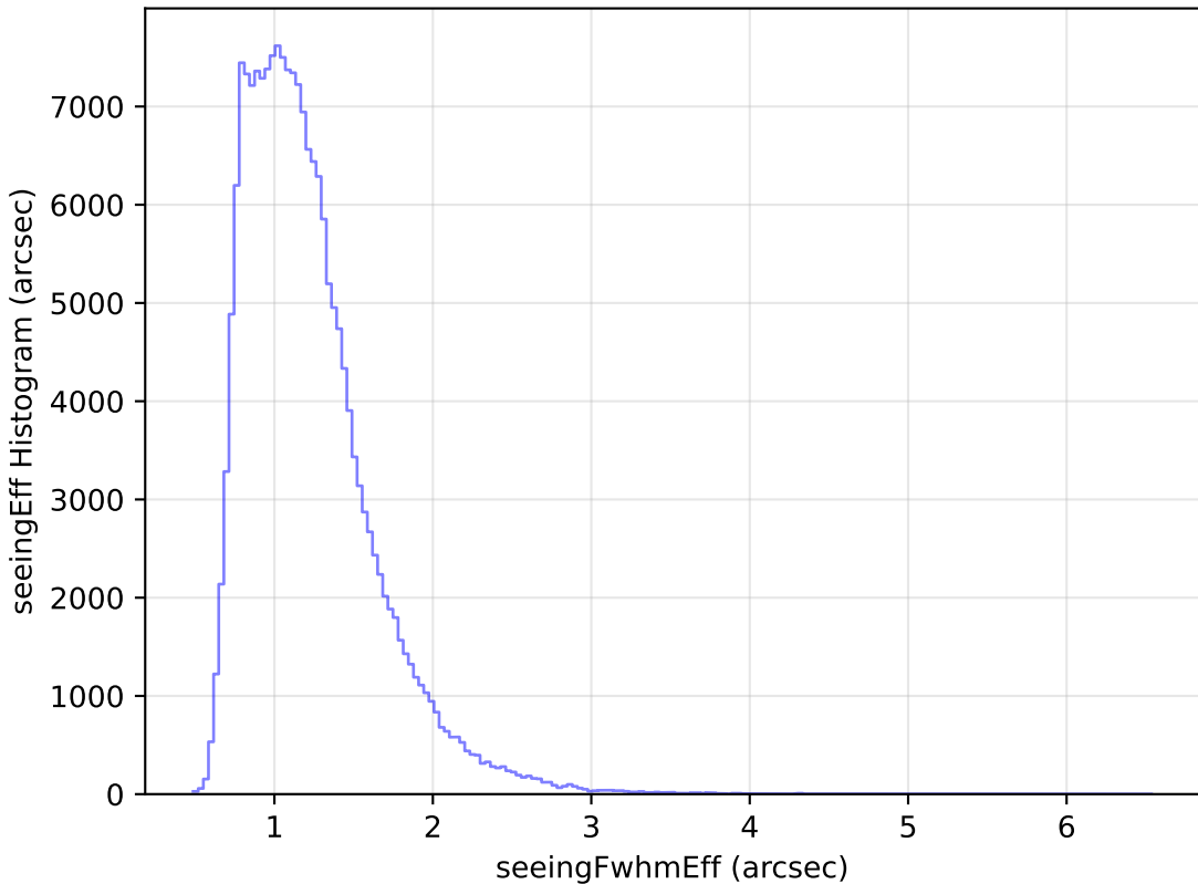
too_elab_r64_d3_gz_v3.4_10yrs All sky g band: seeingEff Histogram
