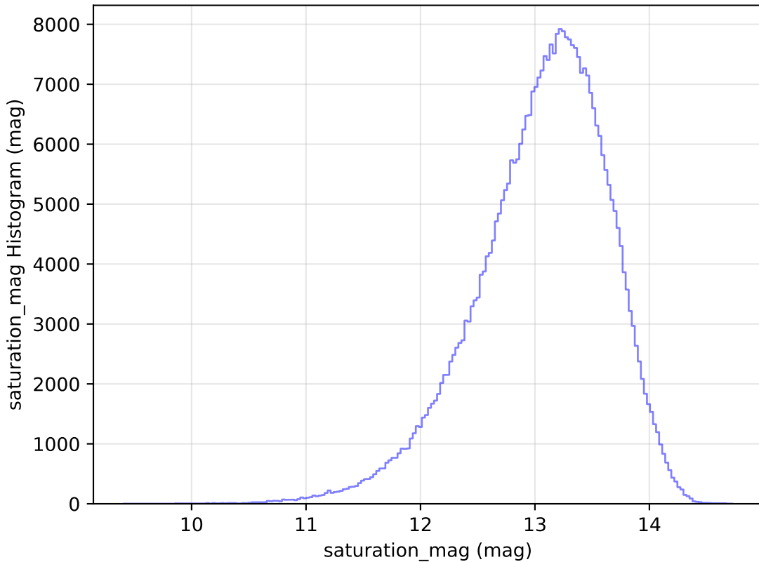
too_elab_r64_d3_gz_v3.4_10yrs WFD y band: saturation_mag Histogram
