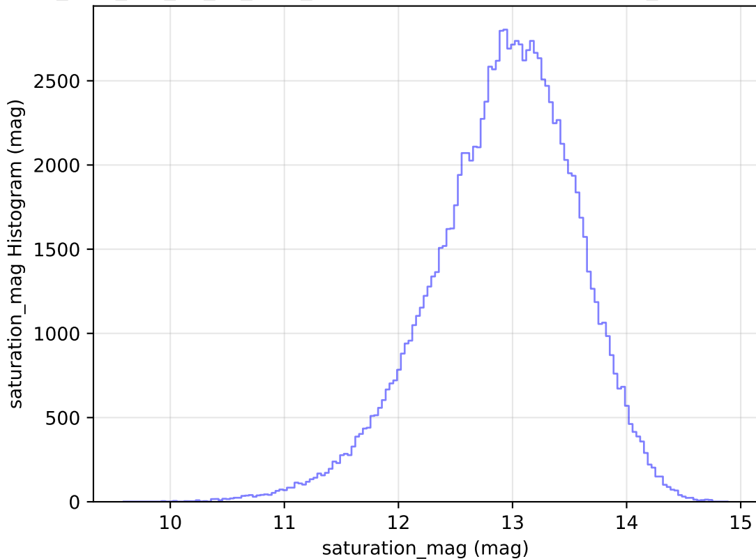
too_elab_r64_d3_gz_v3.4_10yrs WFD u band: saturation_mag Histogram
