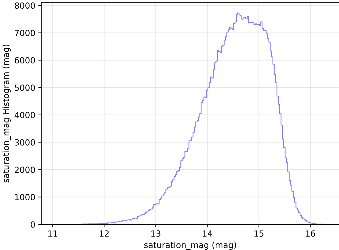
too_elab_r64_d3_gz_v3.4_10yrs WFD r band: saturation_mag Histogram
