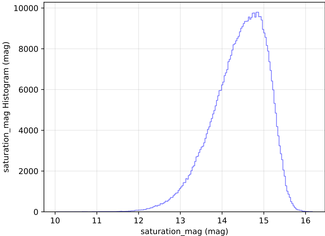
too_elab_r64_d3_gz_v3.4_10yrs WFD i band: saturation_mag Histogram
