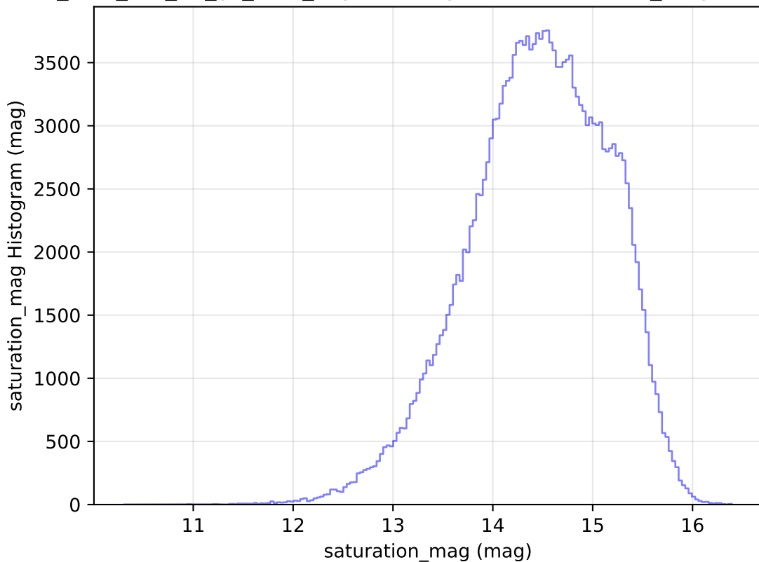
too_elab_r64_d3_gz_v3.4_10yrs WFD g band: saturation_mag Histogram
