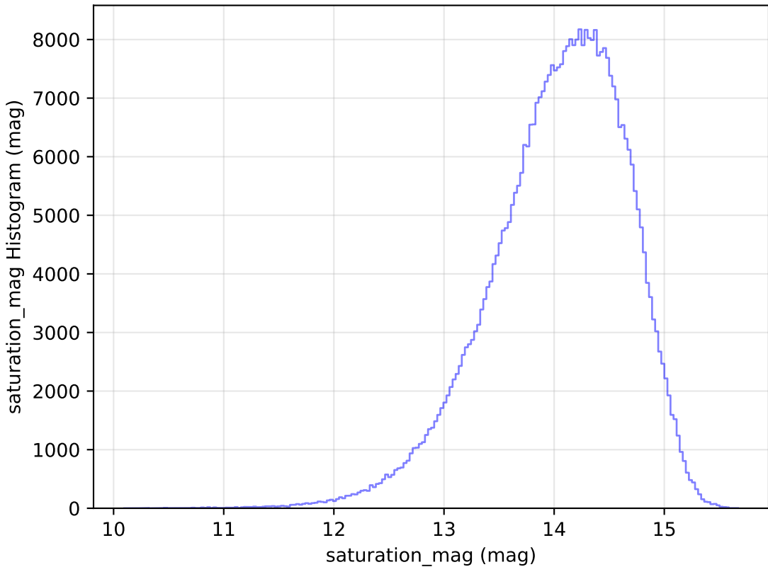
too_elab_r64_d3_gz_v3.4_10yrs All sky z band: saturation_mag Histogram
