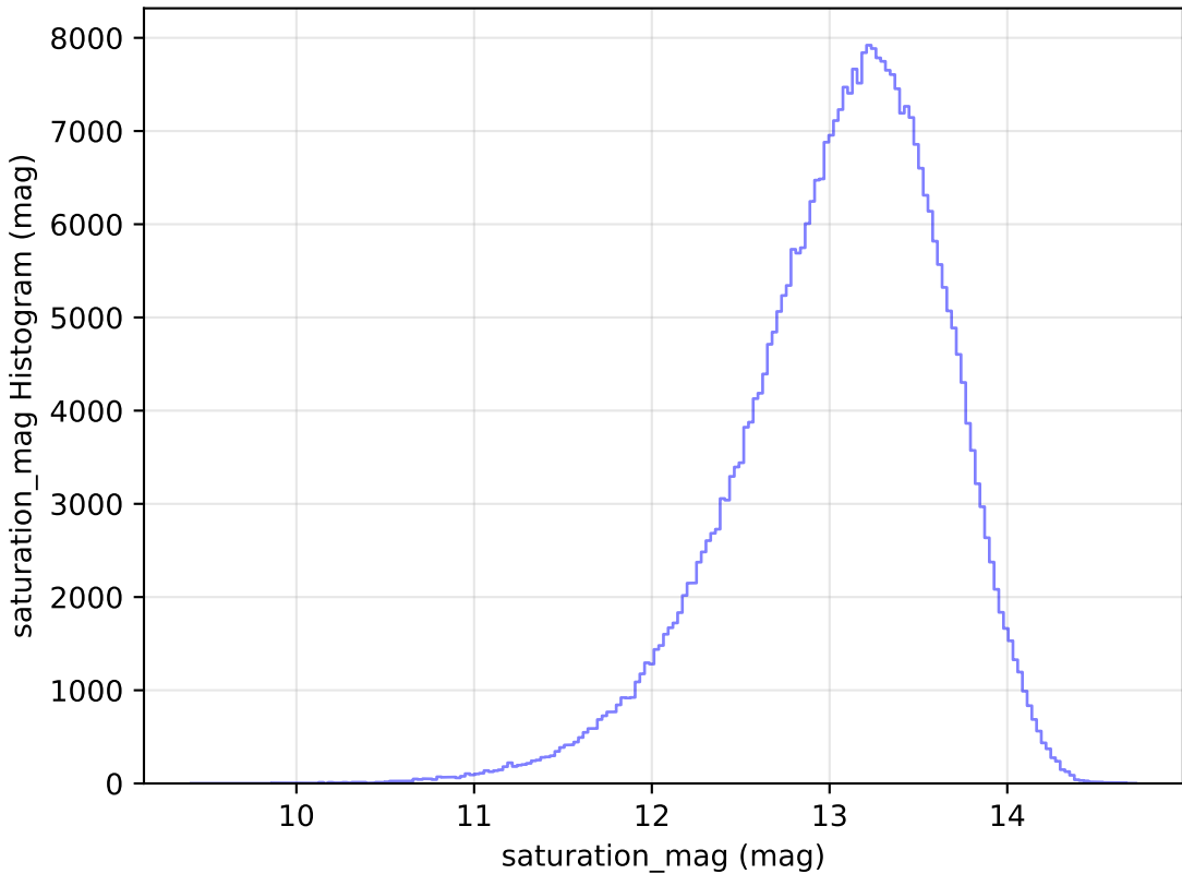
too_elab_r64_d3_gz_v3.4_10yrs All sky y band: saturation_mag Histogram
