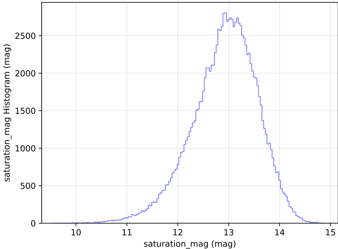
too_elab_r64_d3_gz_v3.4_10yrs All sky u band: saturation_mag Histogram
