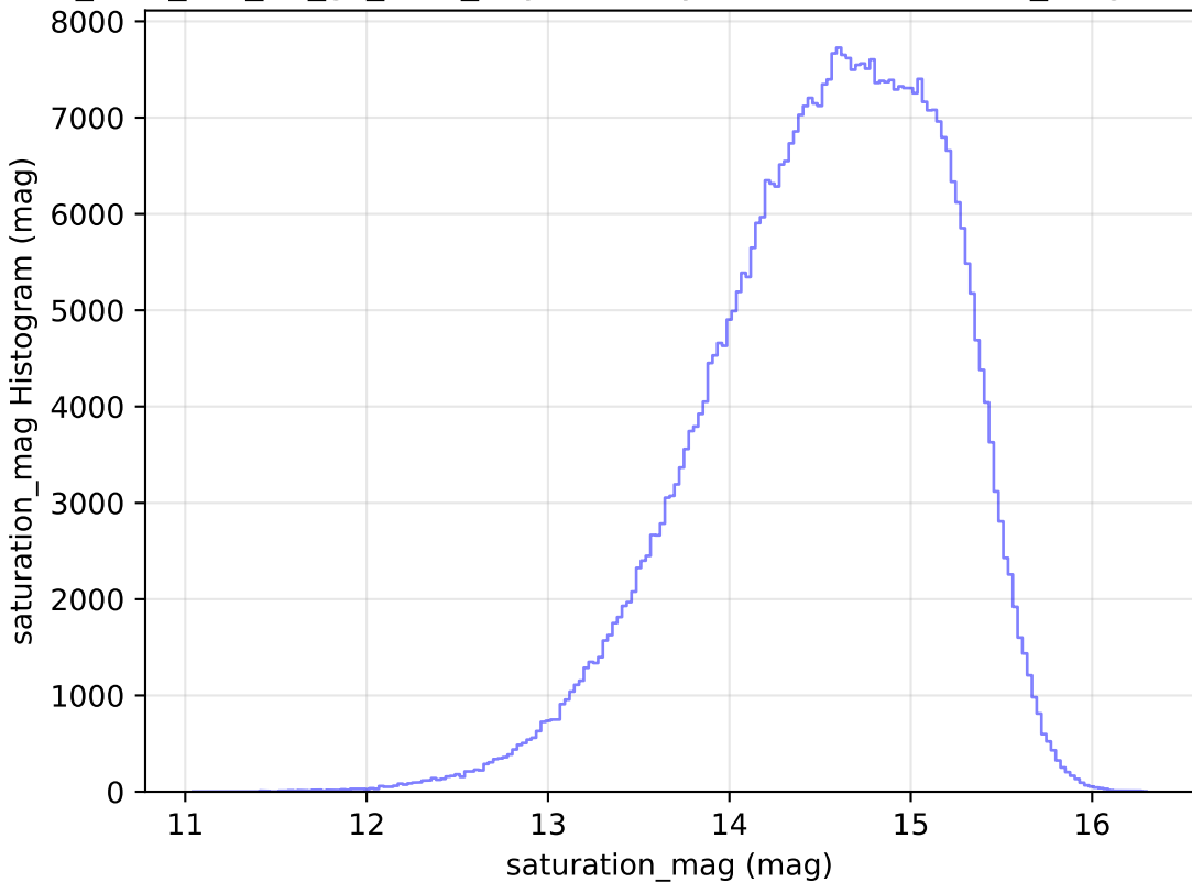
too_elab_r64_d3_gz_v3.4_10yrs All sky r band: saturation_mag Histogram
