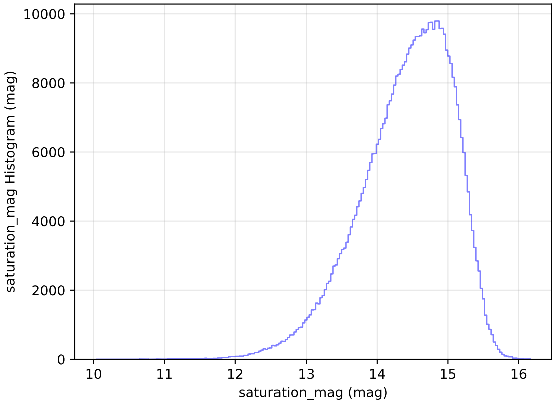
too_elab_r64_d3_gz_v3.4_10yrs All sky i band: saturation_mag Histogram
