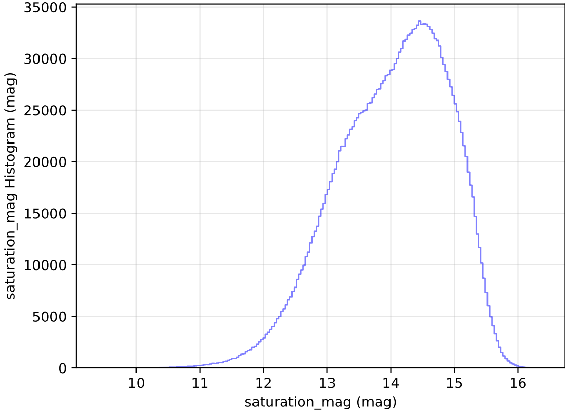
too_elab_r64_d3_gz_v3.4_10yrs All sky all bands: saturation_mag Histogram
