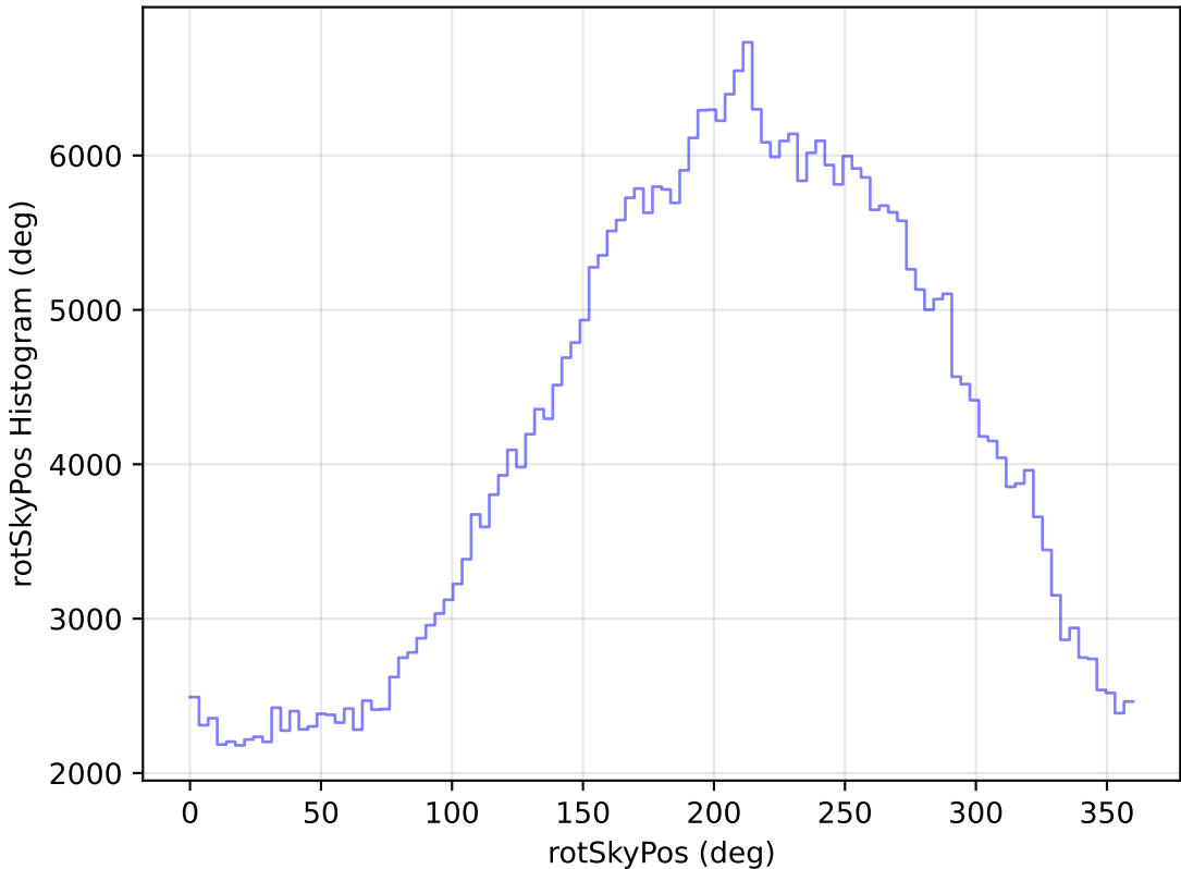
too_elab_r64_d3_gz_v3.4_10yrs WFD z band: rotSkyPos Histogram
