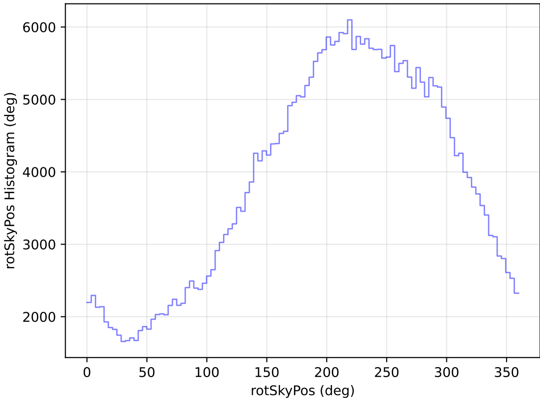
too_elab_r64_d3_gz_v3.4_10yrs WFD y band: rotSkyPos Histogram
