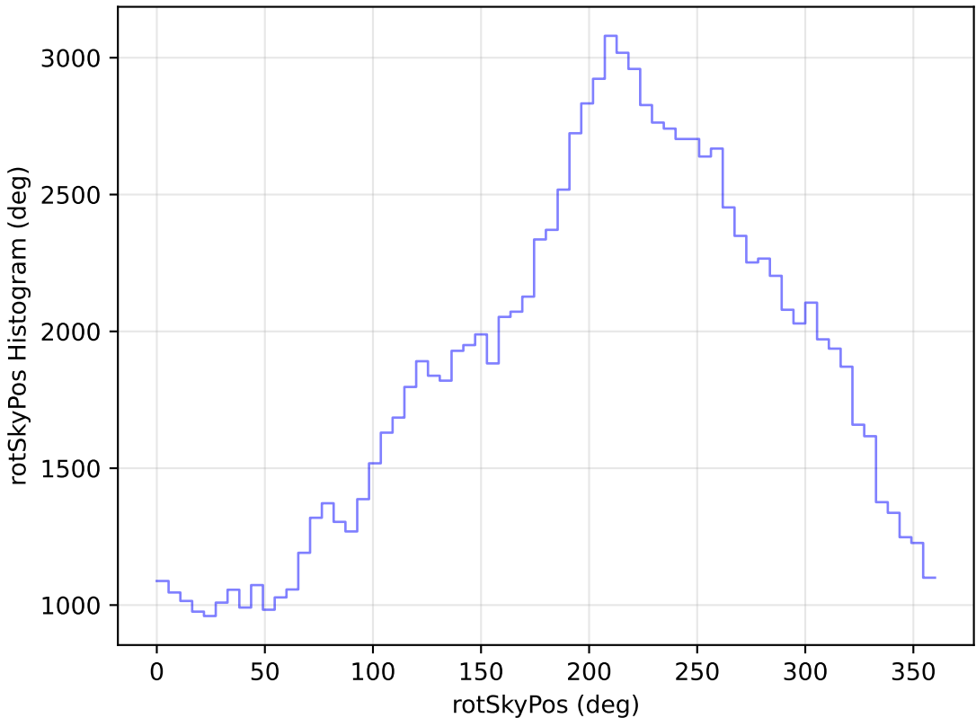
too_elab_r64_d3_gz_v3.4_10yrs WFD u band: rotSkyPos Histogram
