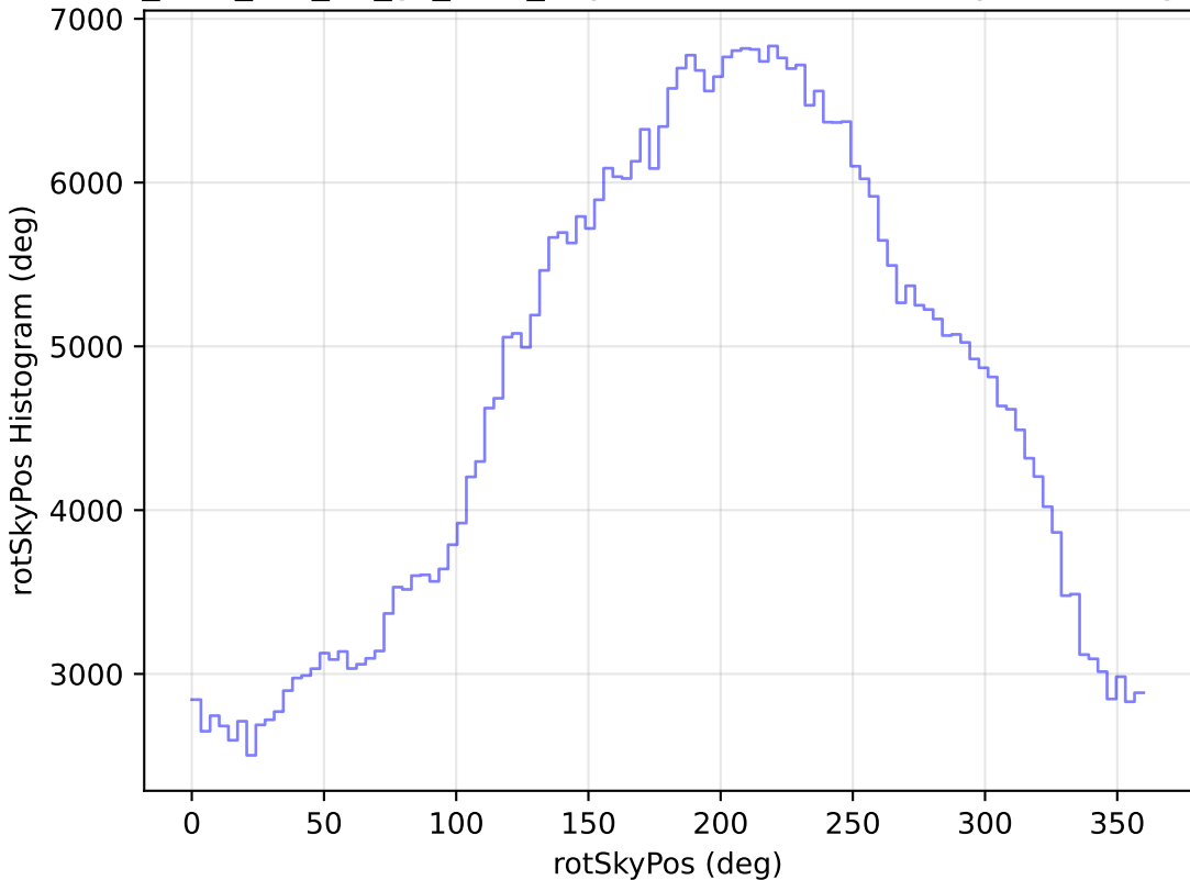
too_elab_r64_d3_gz_v3.4_10yrs WFD r band: rotSkyPos Histogram
