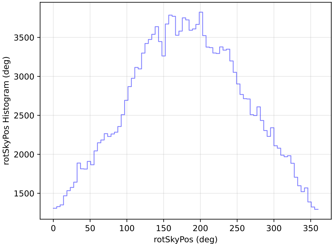
too_elab_r64_d3_gz_v3.4_10yrs WFD g band: rotSkyPos Histogram
