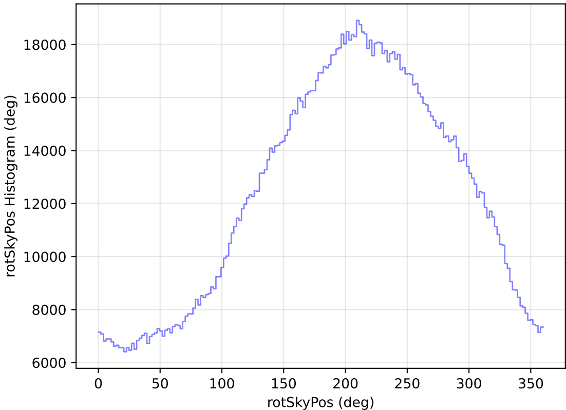
too_elab_r64_d3_gz_v3.4_10yrs WFD all bands: rotSkyPos Histogram
