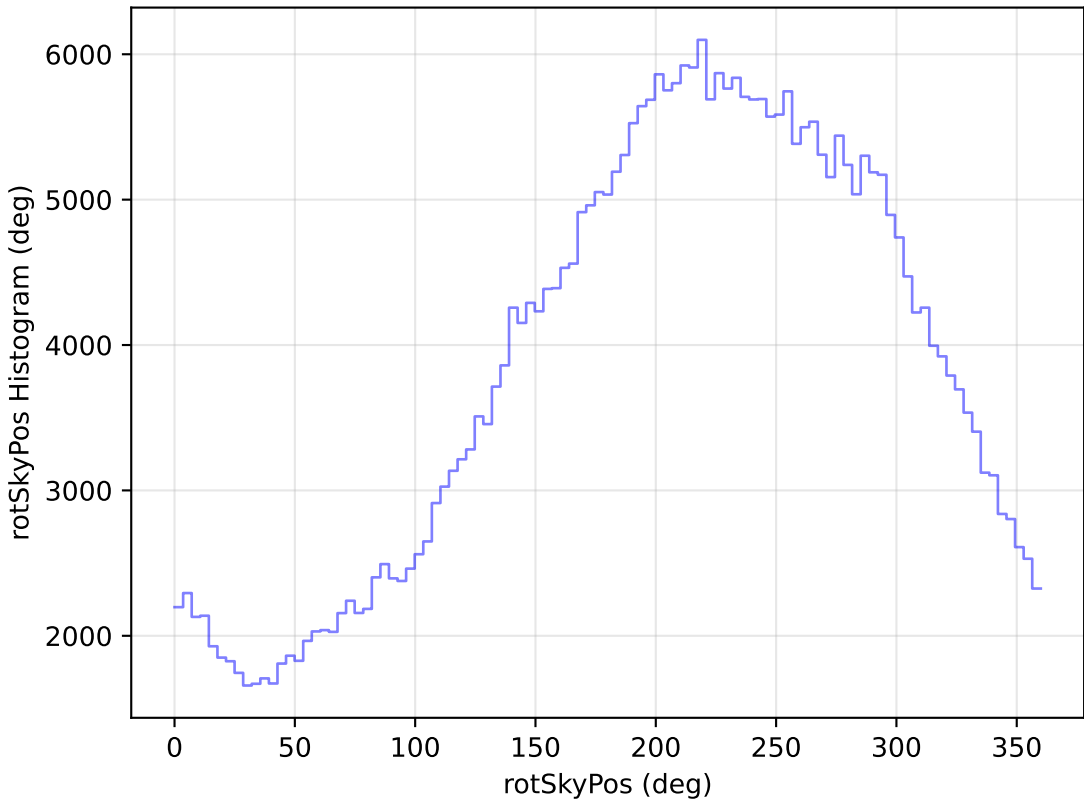
too_elab_r64_d3_gz_v3.4_10yrs All sky y band: rotSkyPos Histogram
