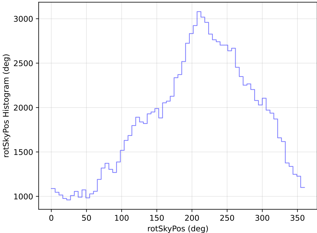
too_elab_r64_d3_gz_v3.4_10yrs All sky u band: rotSkyPos Histogram
