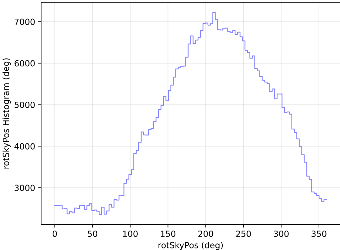
too_elab_r64_d3_gz_v3.4_10yrs All sky i band: rotSkyPos Histogram
