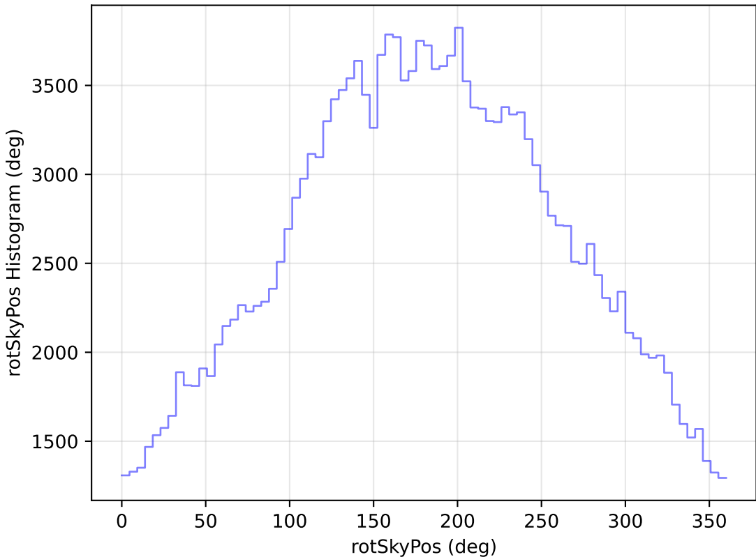
too_elab_r64_d3_gz_v3.4_10yrs All sky g band: rotSkyPos Histogram
